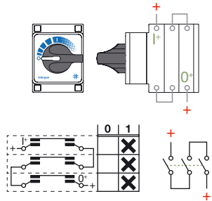
TFV1030 1 polo / 3 pisos 1 2 3 4 5 6 7 8 9 10 11 12 TFV1030
