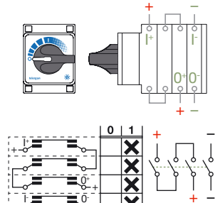
TFV1031 2 polos / 3 pisos 1 2 3 4 5 6 7 8 9 10 11 12 TFV1031
