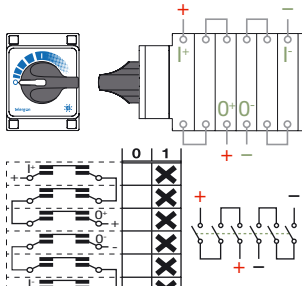
TFV1033 2 polos / 6 pisos 1 2 3 4 5 6 7 8 9 10 11 12 TFV1033
