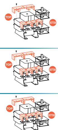
Terminal shrouds (On front switch only)
