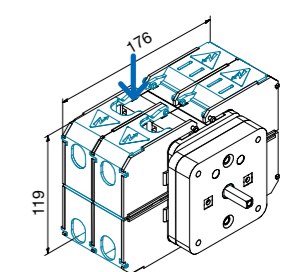
Terminal shrouds (S) Code DT-90028 (4 units)
