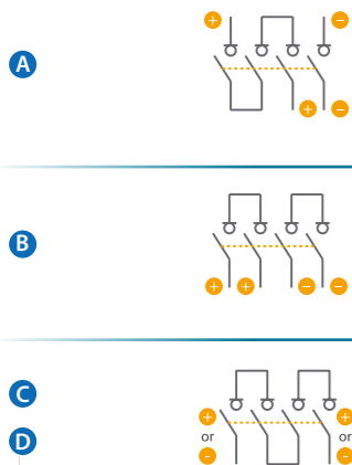
Connection diagram
